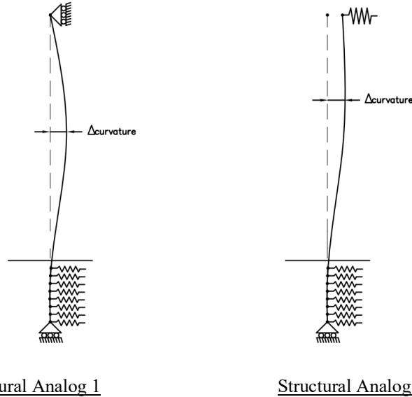
Figure 6.1 Structural Analogs for a Typical Post Frame Column
